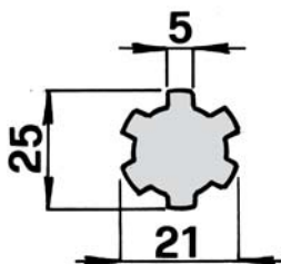
21 UNI221 Z=6
