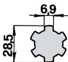
1"1/8 Z=6
