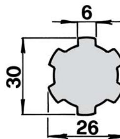
26 UNI220 Z=6
